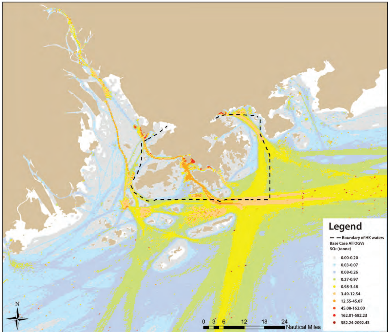
FIGURE 21 Spatial distribution of OGV SO 2 (2008) 19
