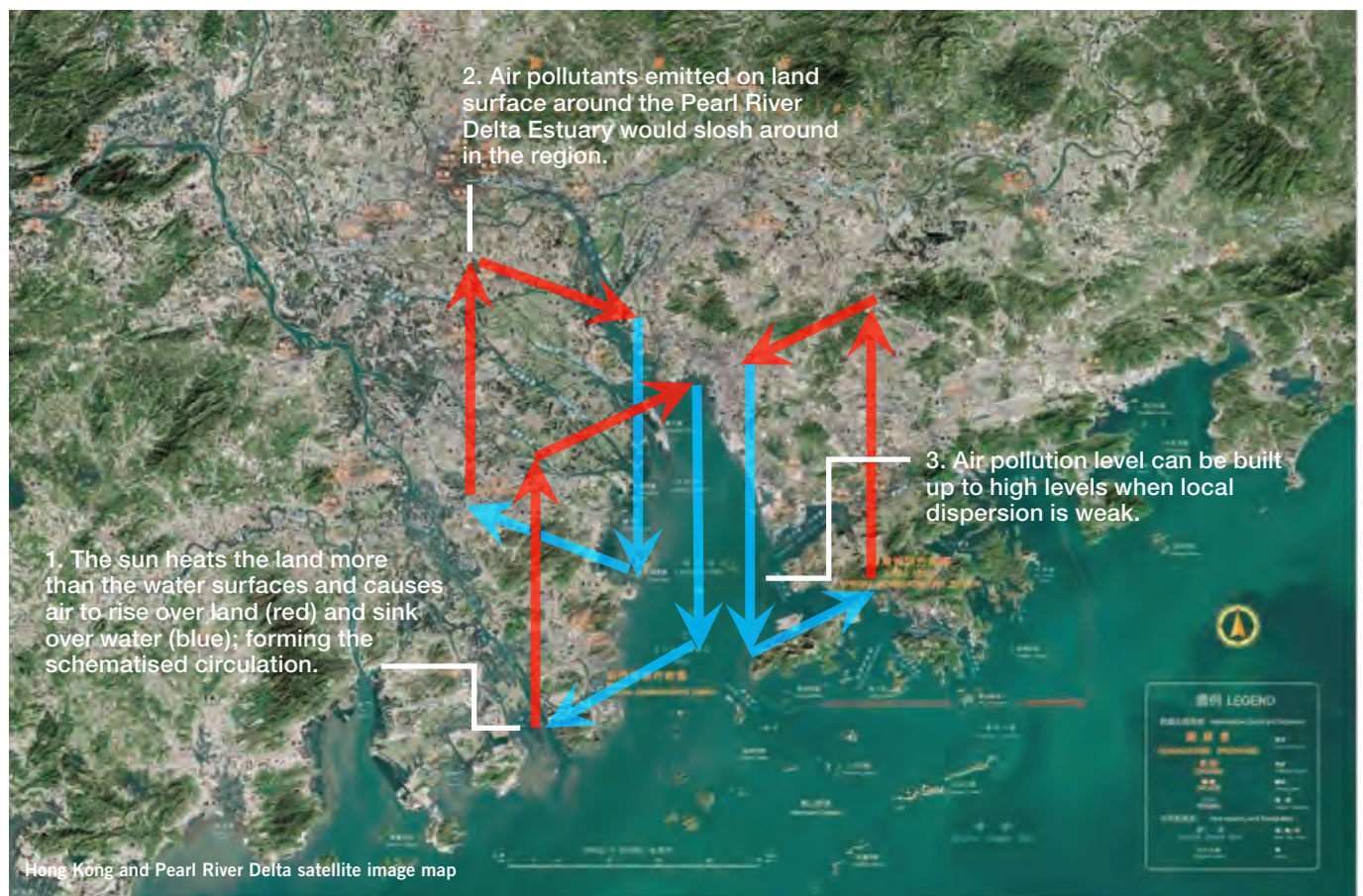
FIGURE 1 Land-sea breeze trapping effect in the HK-Macao-PRD region
